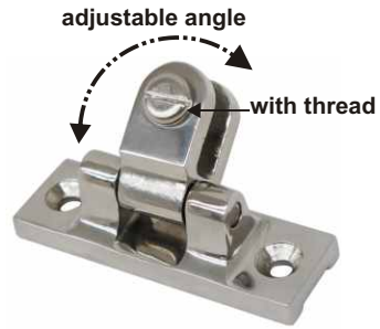
UNIVERSAL DECK HINGE casted AISI 316 ITEM NO. Base Weight/g B19-009 62x21mm(2-5/8"x1-1/8") 100
