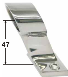
120° FORWARD HANDRAIL FITTING casted AISI 316 ITEM NO. Tube O.D. Weight 009648 22mm(7/8") 140g
