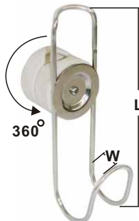
HOOK AISI 304 fit \Phi 25mm tube rail ITEM NO. L mm W mm Weight/g 003017 200 50 220
