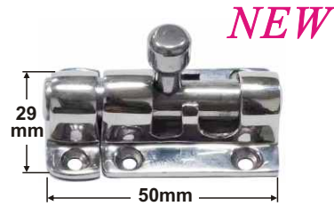
STAINLESS BARREL BOLTS precision casted AISI 316 ITEM NO. Overall B23-029 50mmx29mm
