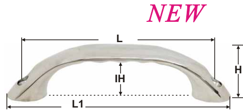
HANDLE AISI 316 ITEM NO. L mm L1 mm IH mm H mm Weight/g B23-026 141 170 32 40 230
