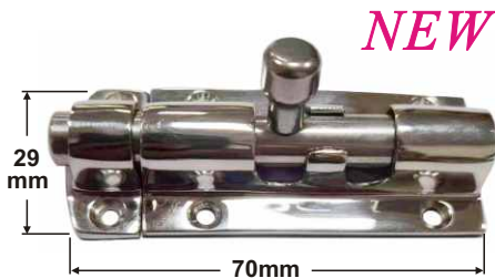
STAINLESS BARREL BOLTS precision casted AISI 316 ITEM NO. Overall B23-030 70mmx29mm
