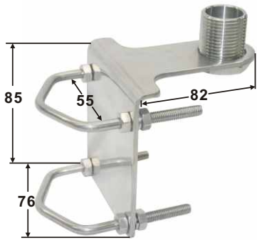
90° ANTENNA MOUNT stamped AISI 304 for TV, VHF, Ioran and GPS antennas ITEM NO. Thread fit Tube Maximum B16-011 1"-14 \Phi 55mm
